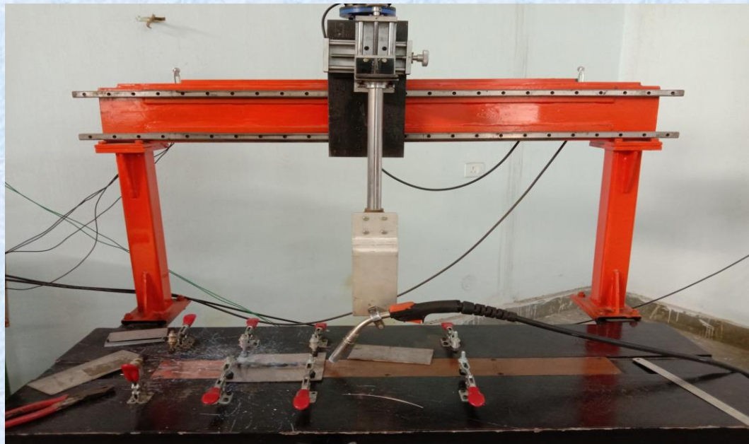
Metal Inert Gas Welding Automatic Setup
